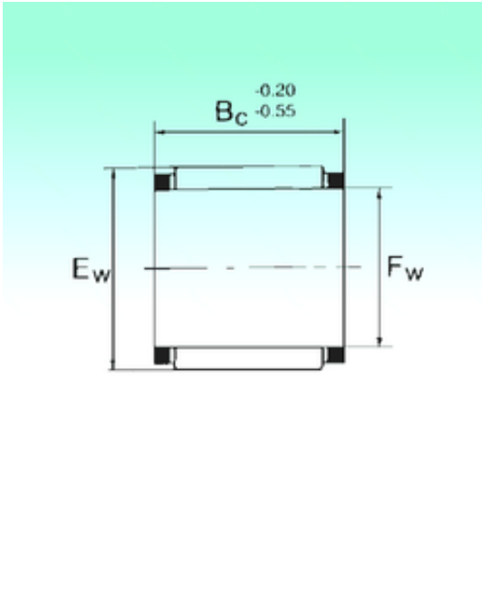
KBK 15x19x19 Bearing 2D drawings and 3D CAD models
